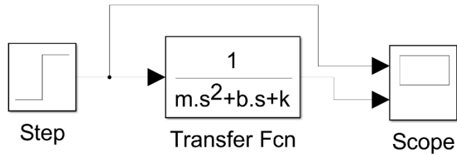
Gambar 3. 19 Diagram Blok
